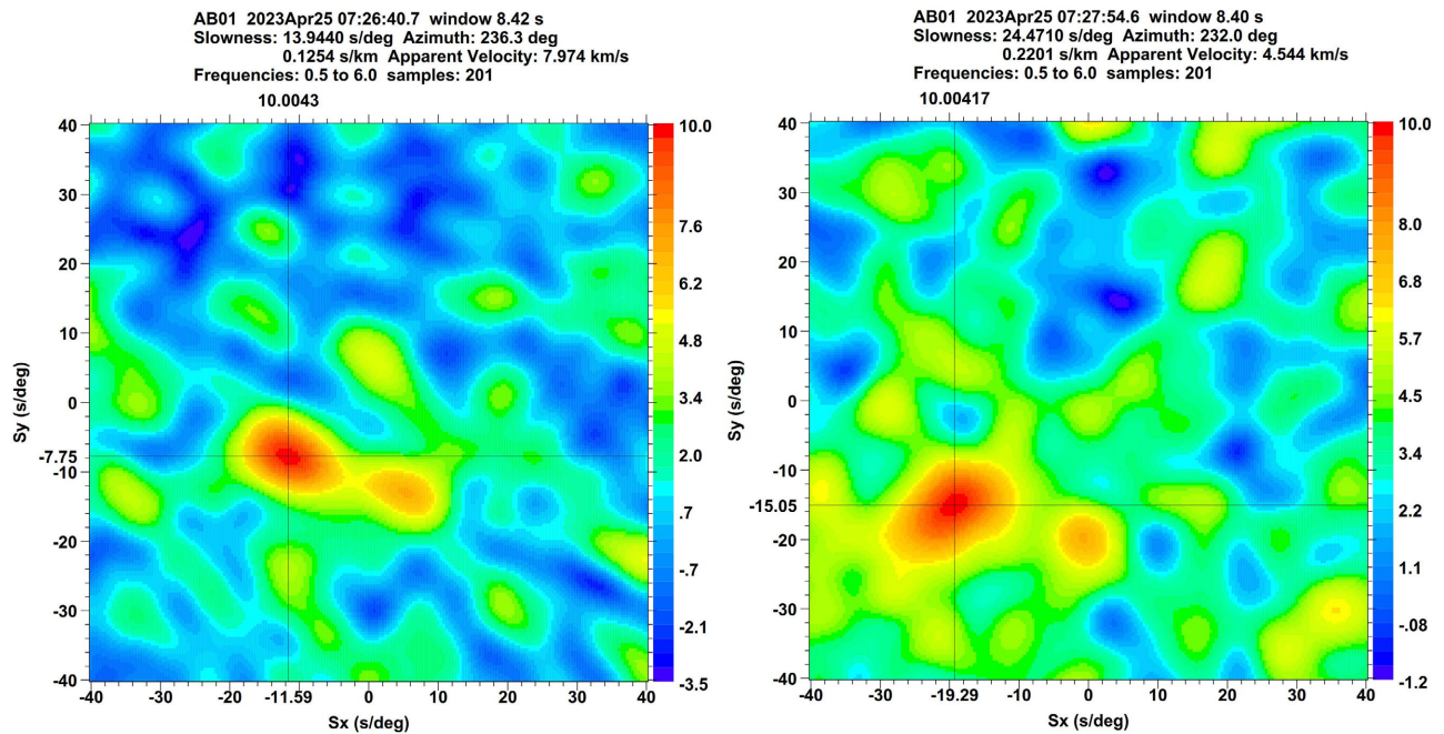
Figure 3. Results of F-k-analysis by P-wave (left) and S-wave (right) from Akbulak seismic array.
